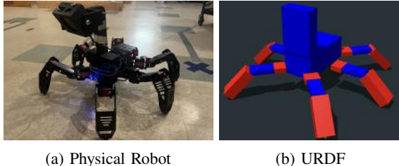
Fig. 2: (a): The SpiderPi hexapod robot used in our work, with Intel L515 and T265 mounted onboard. (b): URDF model of SpiderPi robot we create for training.
